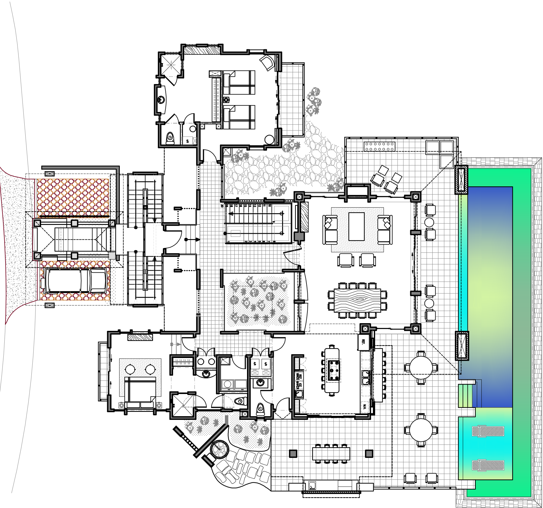
FLOOR PLANT LEVEL 0±0.00 ESC 1 : 75
