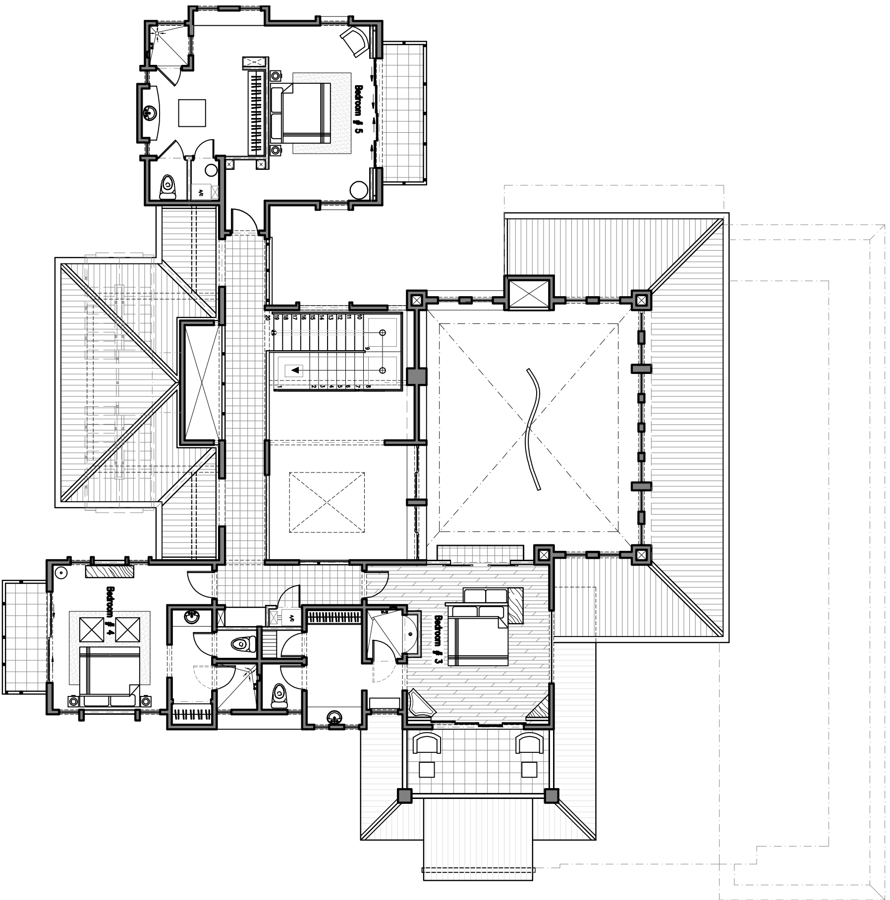
FLOOR PLANT LEVEL 0+3.50 m ESCALA 1 : 75
